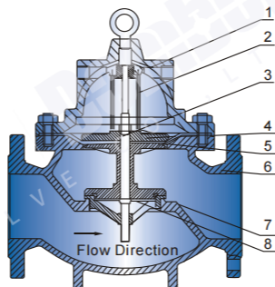
FIG.1-Diaphragm type
