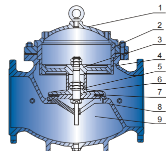
FIG.2-Piston type
