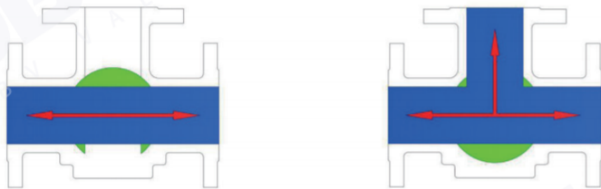
T 型三通球阀 NO.1
